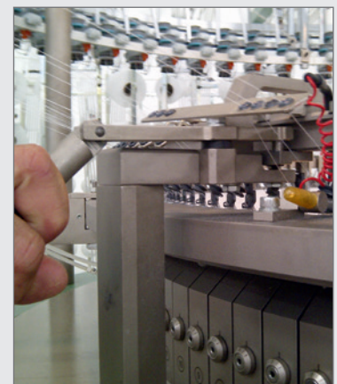
click clack system on yarn carrier ring (patented)
